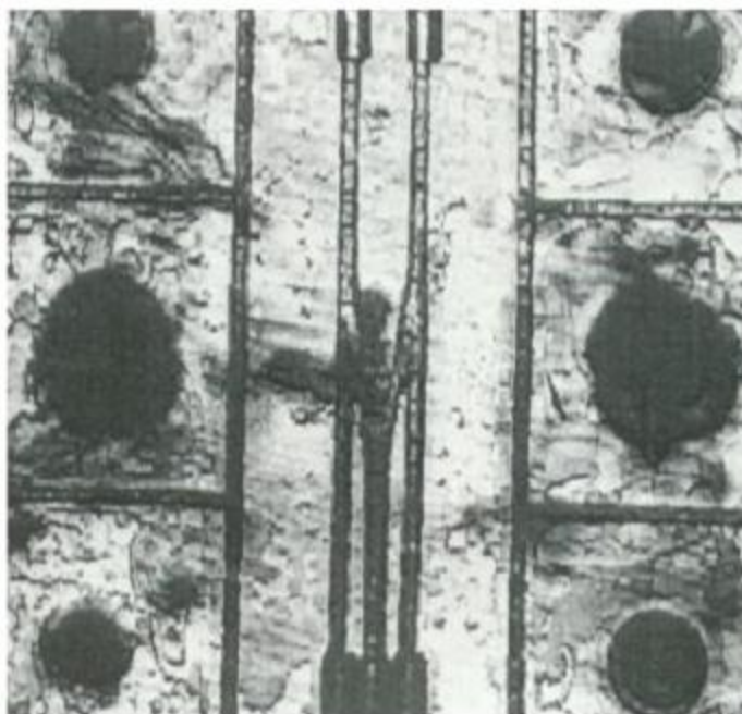
Frequency 60 MHz, Image width: 30 mm, Thickness of aluminium lamella: 2mm
